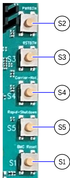
Figure 38: Button Switches
