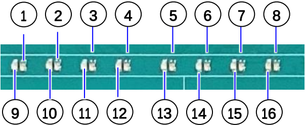
Figure 41: SFP28 LEDs
