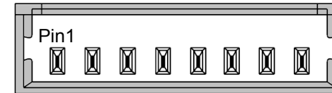
Power Connector X20
