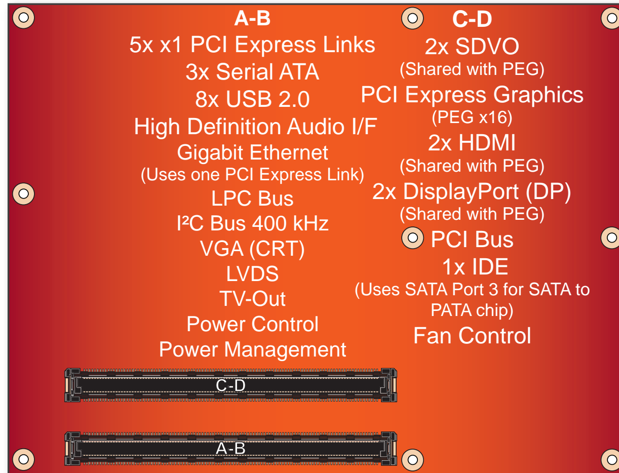
top view
